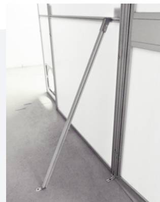
Truss Brace Truss Braces help to secure a longer length of panels by bracing them from mid-panel, then fastening the bracket to the floor.
