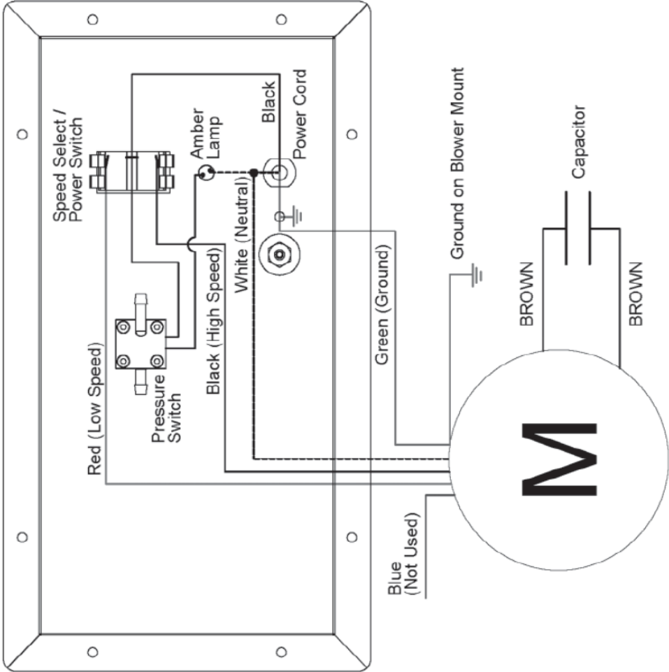
H2KM Control Panel Wiring Diagram
