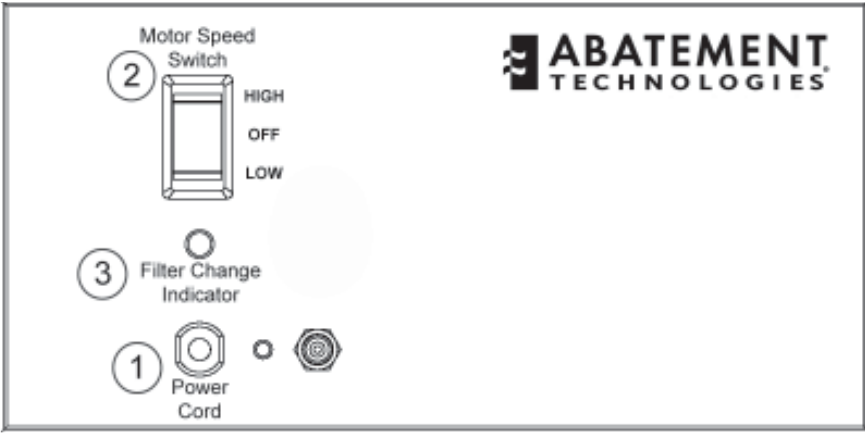
H2KM Control Panel
